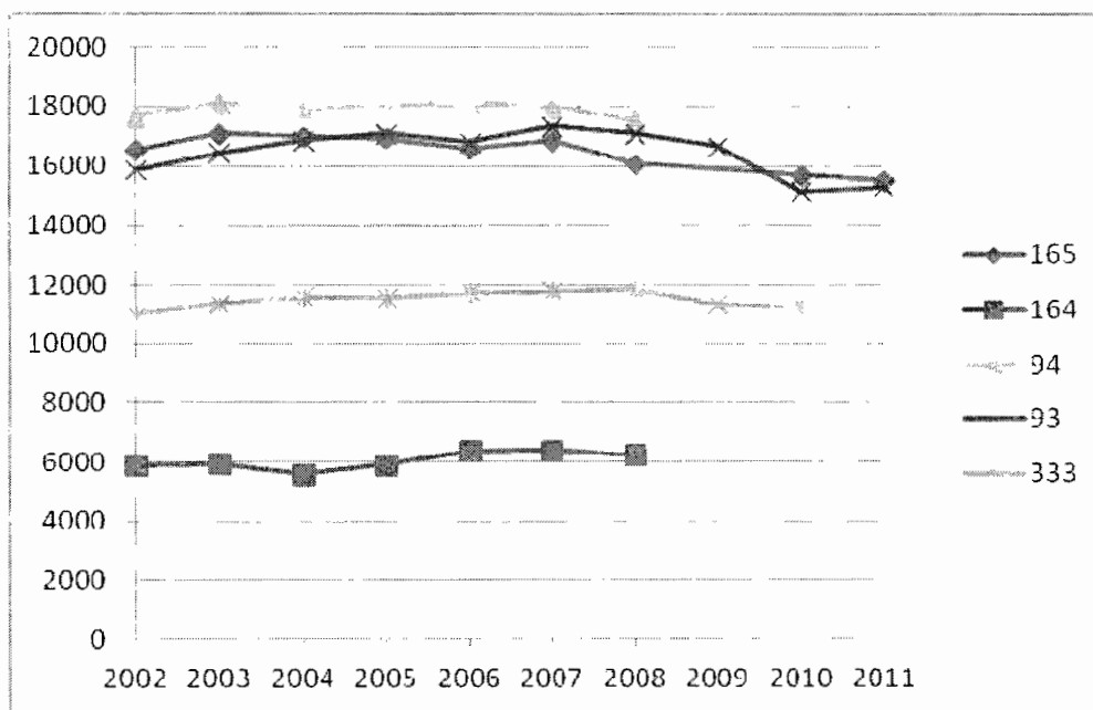
Figure 3.8: Year-to-year comparison of two-way AADTs (in vehicle/day)
