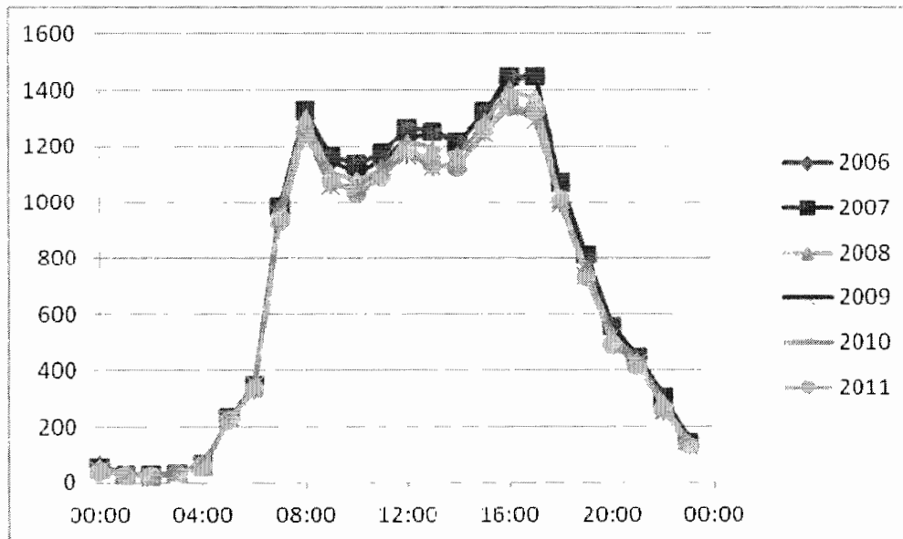
Figure 3.11: Weekday Two-Way Daily Profiles for Site 165
