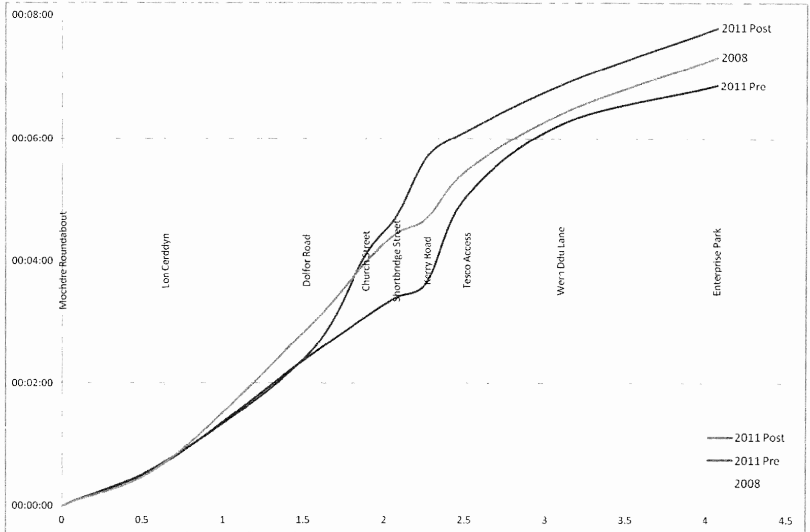
Figure 3.3: Eastbound cumulative journey time against cumulative journey distance (in km)
