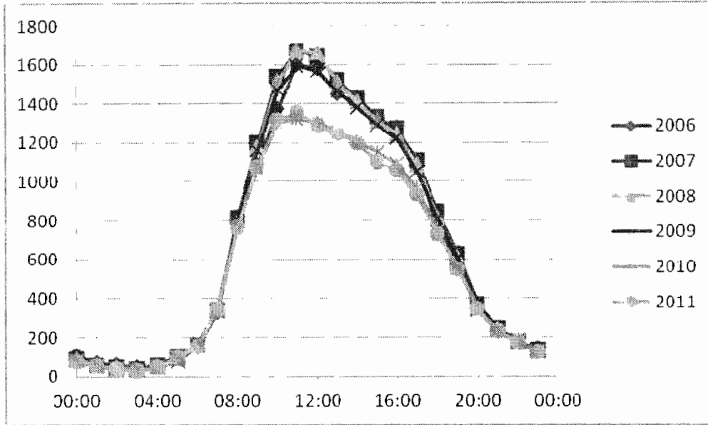
Figure 3.12: Saturday Two-Way Daily Profiles for Site 93
