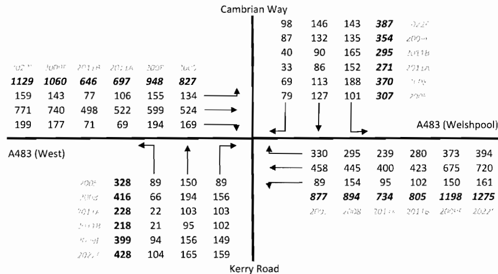
Figure 3.5: Weekday PM peak turning movements (in vehicles/hour)
