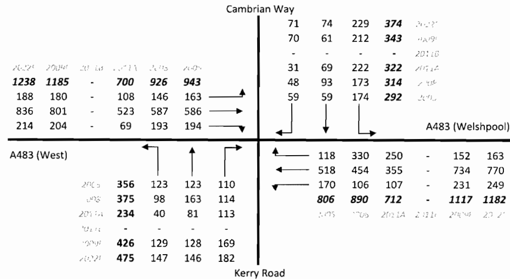
Figure 3.6: Saturday peak turning movements (in vehicles/hour)
