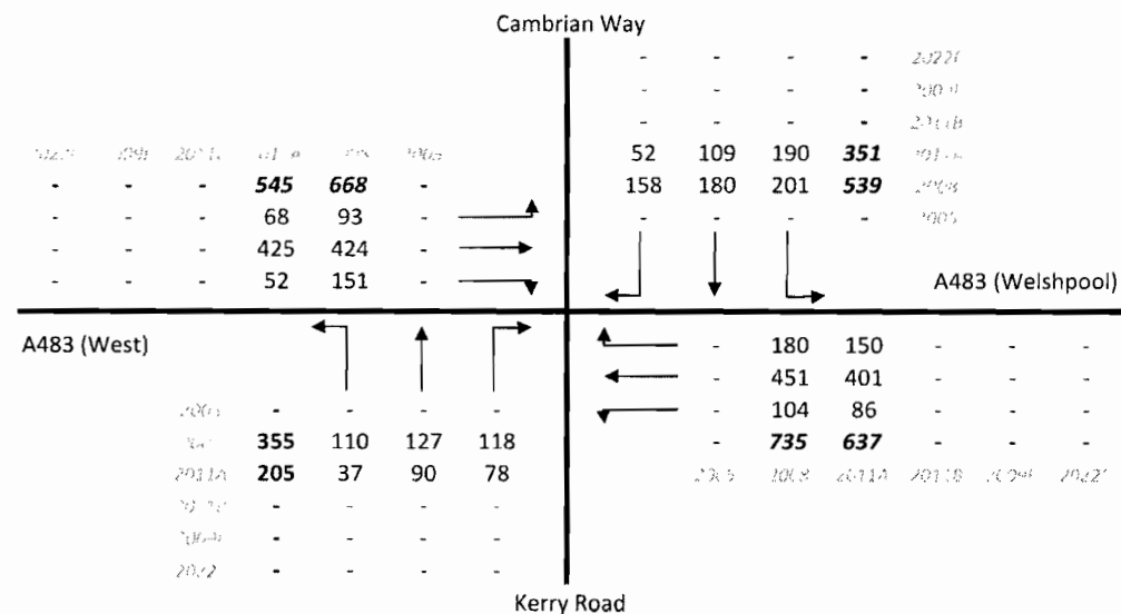
Figure 3.4: Weekday AM peak turning movements (in vehicles/hour)
